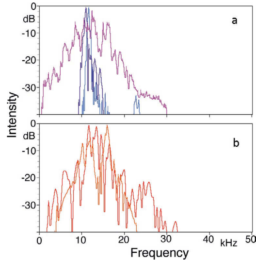
Fig. 8. Power spectra of sounds of Anaulacomera almdaensis sp. nov.: a , male calling song (blue: two different males) and example of soft song (lila); b , female response (red: two different females).
