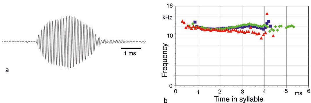
Fig. 7. Anaulacomera almadaensis sp. nov., details of male song: a , time-amplitude pattern of a syllable of the male song; b , cycle-by-cycle frequency of three syllables of one echeme.
