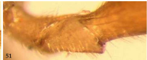
Figs 50–51. A. striatum (Brischke) ♀: 50. Hind metatarsus; 51. Hind trochanter.
