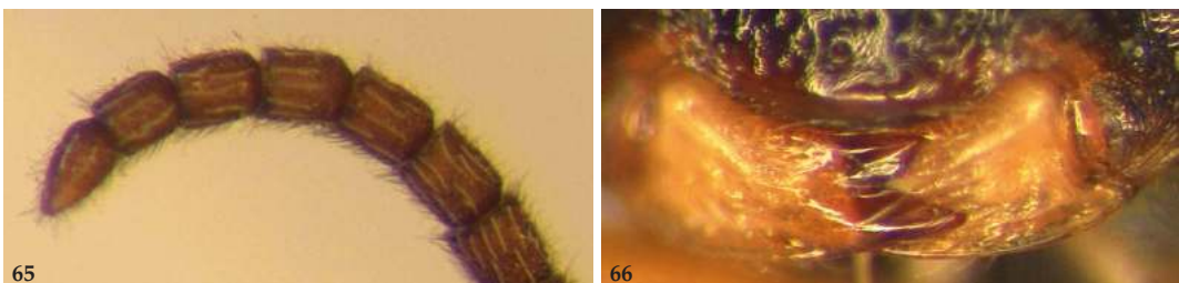
Figs 65–66. 65. Apical flagellomeres of A. flagellator spec. nov.; 66. Mandible of A. italicum Schwenke ♀, Arrow shows larger lower tooth.
