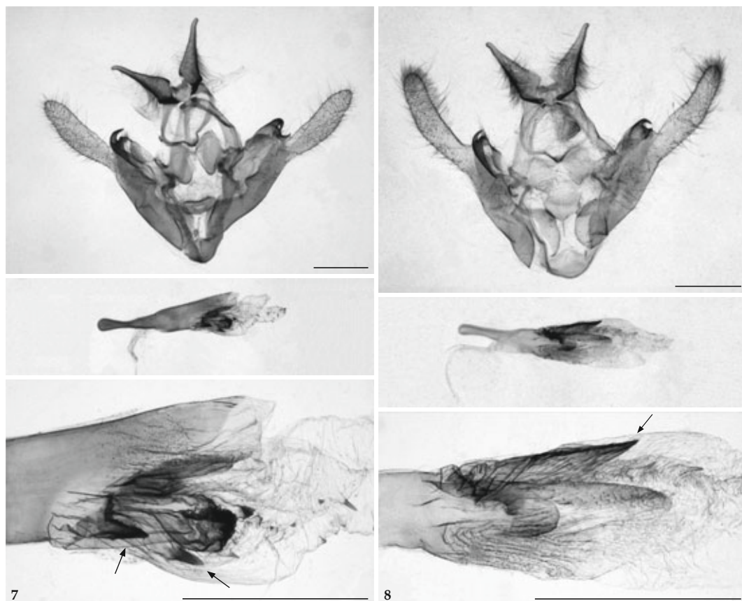
Figs 7-8. Male genitalia, aedeagus, and magnified detail of aedeagus. Scale bars = 1 mm. 7 , Hypobapta tachyhalotaria sp.n., holotype, prp. ZSM G 13974. 8 , Hypobapta percomptaria (Guenée, 1858), Tasmania, prp. ZSM G 13972.
