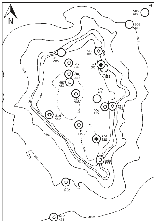
Fig. 1. Map of the Great Meteor Seamount (30°00'N 28°30'W) showing the 19 stations (circles) analysed in the present contribution, including station number and sampling gear. Black rhombuses indicate findings of Zosimeidae, white suns show findings of Zosime anneae sp. nov. Station 505 is located outside the figure (arrow). GKG: Giant Box Corer; EBS: Epibenthic sled; MUC: Multicorer.
